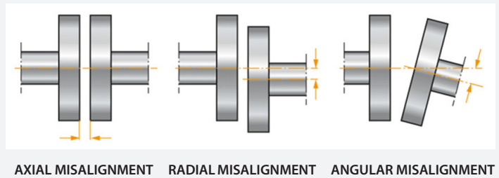
Figure 2: Common Misalignments
