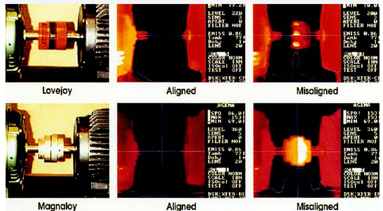
Figure 3: Misalignment Heat Generation
