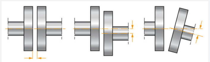
AXIAL MISALIGNMENT RADIAL MISALIGNMENT ANGULAR MISALIGNMENT
